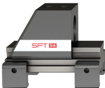
2 SPANNEINHEIT BASISBLOCK + FESTER BASISBLOCK CLAMPING UNIT BASE BLOCK + FIXED BASE BLOCK
